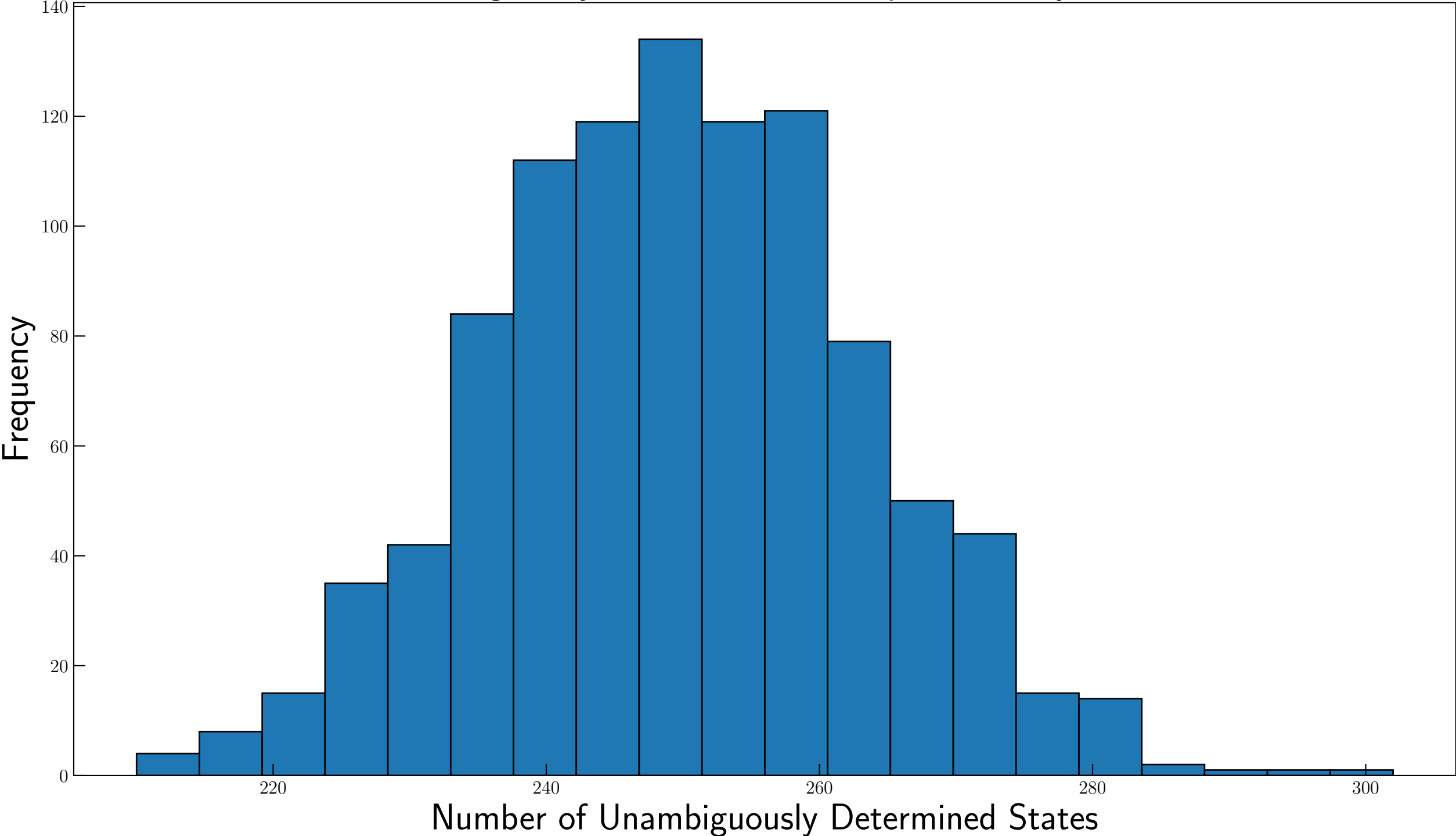
Unambiguously Determined States per Block by Alice
